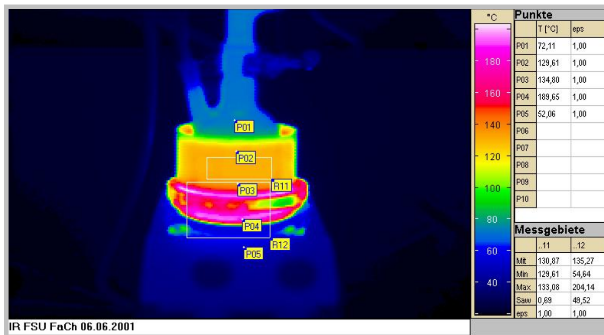
Fig. 1: IR-photo – heating stage with oil bath
